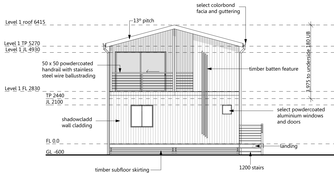
1 Elevation 1 1:100
